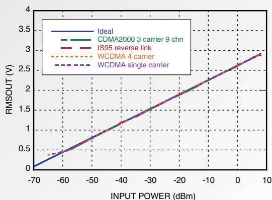
HMC610LP4E RMSOUT vs. Pin with Different Modulations @ 900 MHz
