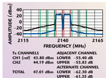
▲ Fig. 1 Corrected and uncorrected ACP results for the TGH2932-FL Doherty configuration.
