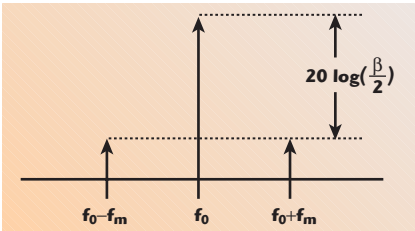
▲ Fig. 3 Spectrum of a single tone PM ( \beta < 1 ).
