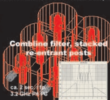
LTCC diplexer
