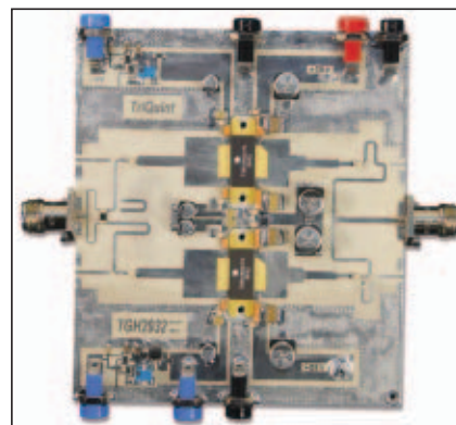
▲ Fig. 2 The TGH2932-FL Doherty evaluation board.
