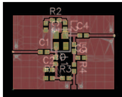
▲ Fig. 5 User-placed internal ports and separate artwork are not needed to perform nonlinear EM co-simulation because of tight EM integration.
