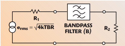
▲ Fig. 2 Calculation of maximum available power.
