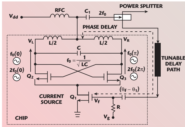
Fig. 15 Self-injected coupled oscillator.
