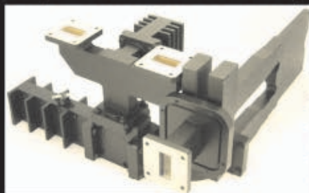
Optimization example: TX arm, HP filter, Magic Tee, double Moreno cross-coupler, waffle filter, dielectric window
