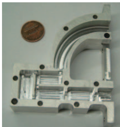
▲ Fig. 3 A 10 GHz bandpass filter in integrated waveguide technology.
